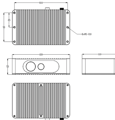
Product Dimensions
